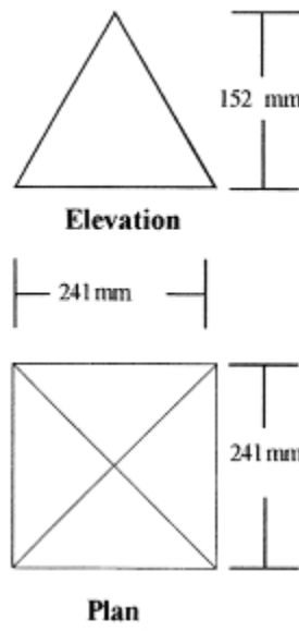
Fig. 1b Plywood Pyramid (PWP)
